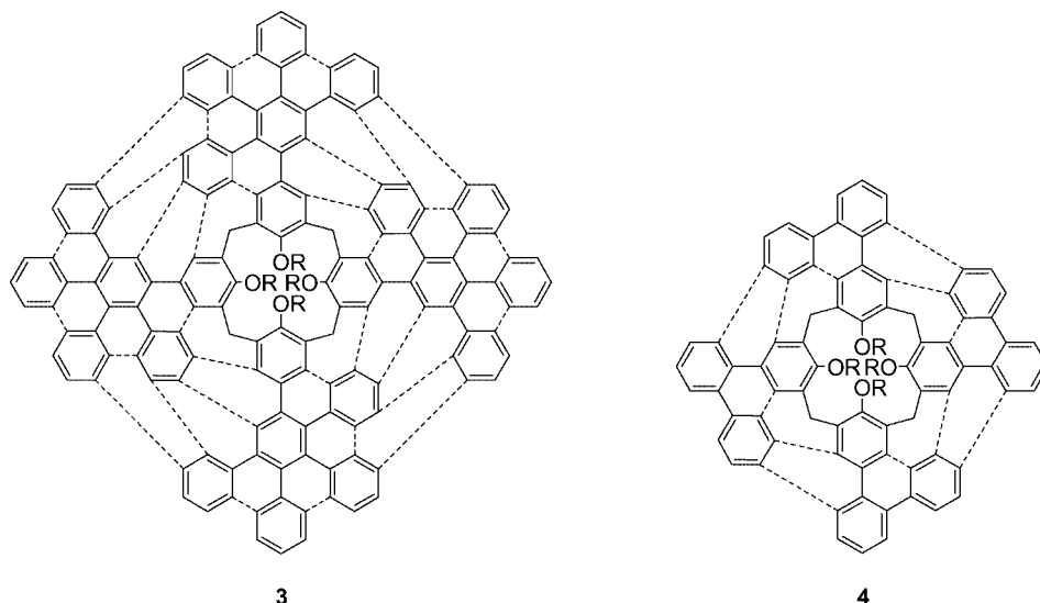
Scheme 1. The polyphenylic calixarenes 3 and 4 as precursors for funnelene syntheses by cyclodehydration. Dashed lines indicate the necessary formation of C–C bonds (R = alkyl).
