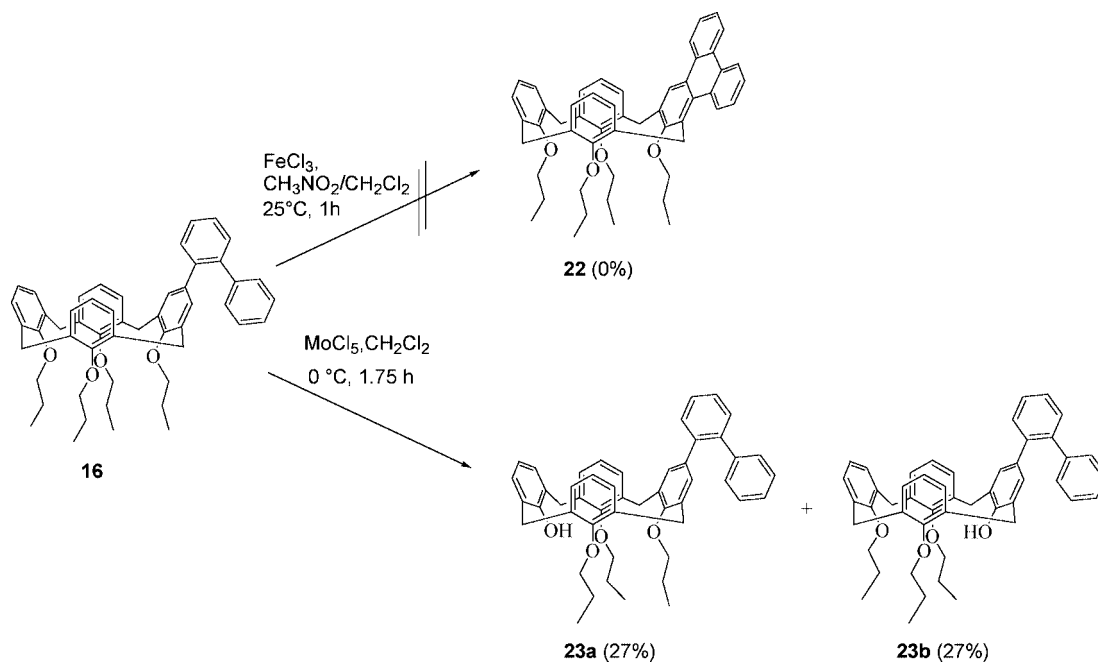
Scheme 7. Preliminary cyclodehydration experiments of 16 to approach the synthesis of an inherently chiral calix[4]triphenylene.
