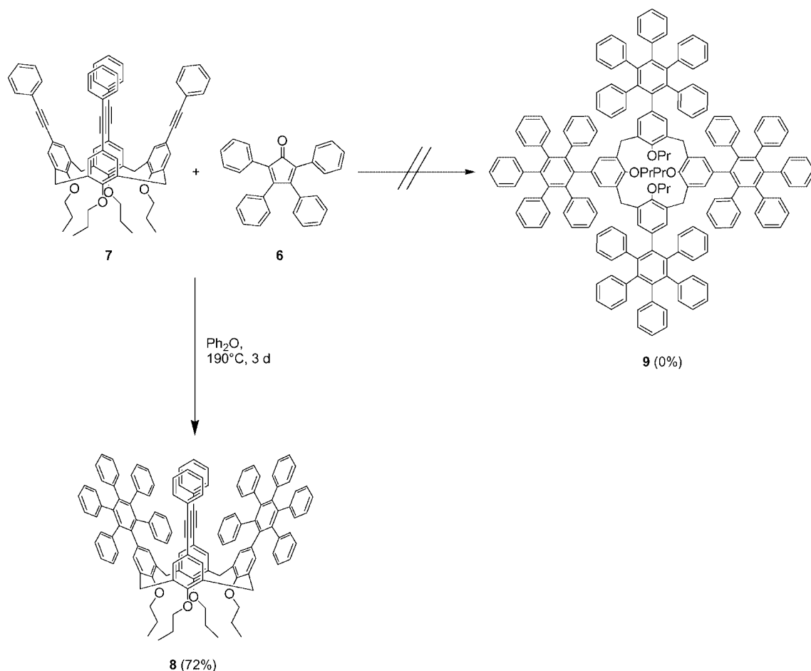
Scheme 3. Diels–Alder reaction of tetrakis(phenylethynyl)calixarene 7 with tetracyclone ( 6 ).
