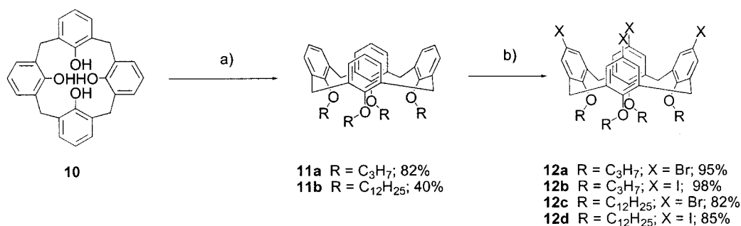
Scheme 4. a) DMF, NaH, RBr, 60–70 °C, 2 h. b) bromination: NBS, 2-butanone, room temperature, 3 d ( 12a ), 24 h ( 12c ); iodination: 1. Ag(OOCCF 3 ), CHCl 3 , 15 min; 2. I 2 , 20 min.
