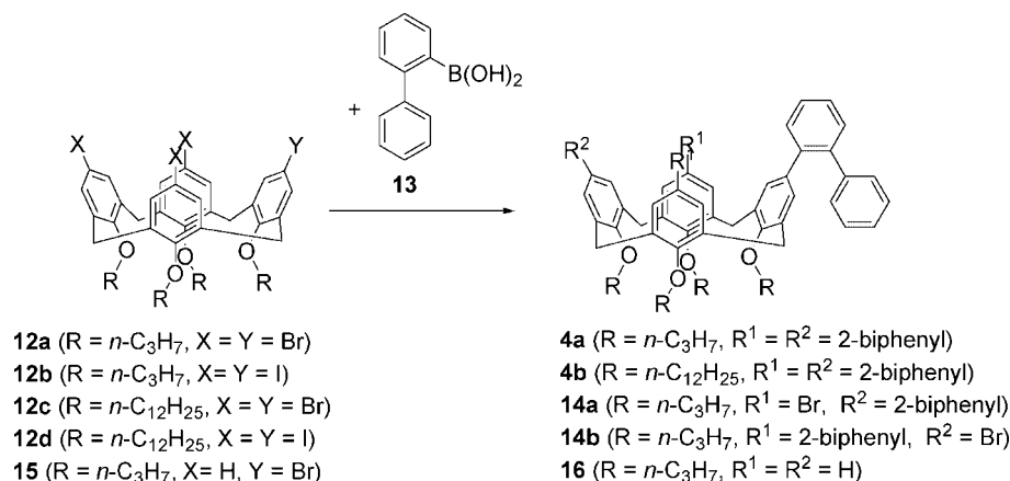
Scheme 5. Suzuki cross-coupling reaction of halocalixarenes 12a–12d with 2-biphenylboronic acid ( 13 ). See Table 1 for conditions and yields.
