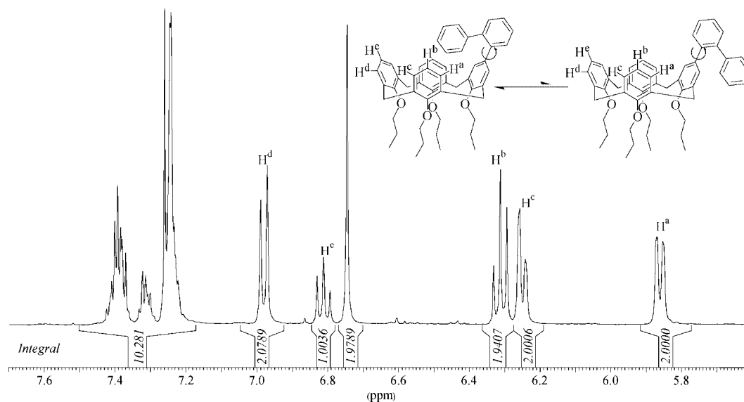
Figure 5. Aromatic region of the ^1\text{H} NMR spectrum of 16 in \text{CDCl}_3 (400 MHz).
