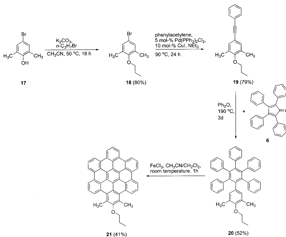
Scheme 6. Synthesis and cyclodehydration of model compound 20 .
