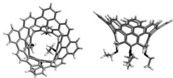
Figure 2. Computer-generated model (MM2-optimised) of the functionalised funnelene 2 .
