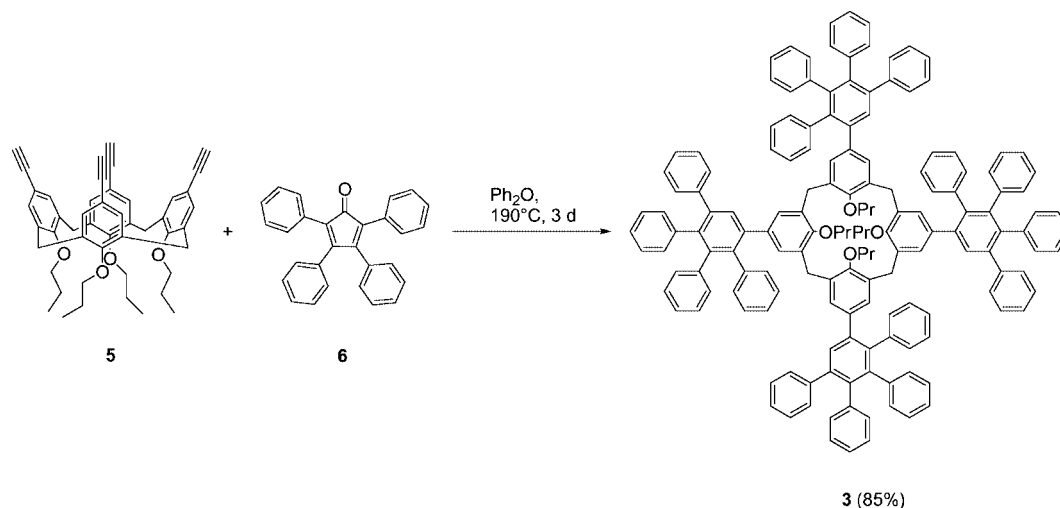
Scheme 2. Diels–Alder reaction of the tetraethynylcalixarene 5 with tetracyclone ( 6 ).
