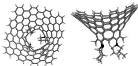
Figure 1. Computer-generated model (MM2-optimised) of the functionalised funnelene 1 .
