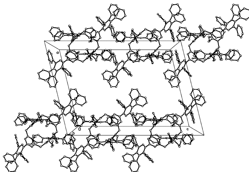
Figure 4. Packing of 3 in the unit cell. View along the crystallographic b -axis. Hydrogen atoms and solvent molecules have been omitted for clarity.
