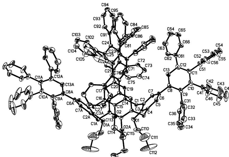
Figure 3. Crystal structure of compound 3 with thermal ellipsoids. Hydrogen atoms have been omitted for clarity.
